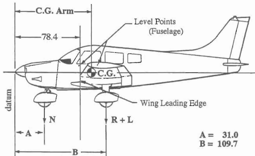
LEVELING DIAGRAM
